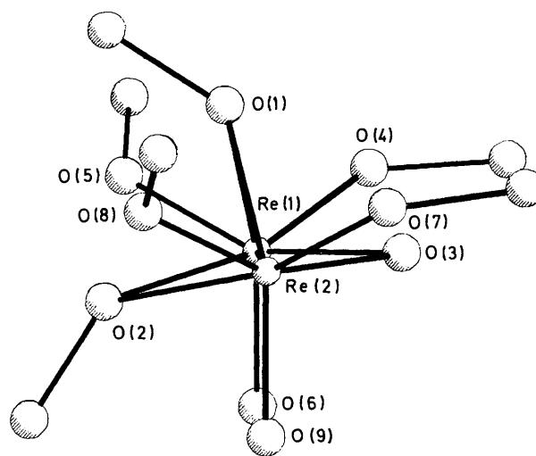
FIGURE 2 View of the \text{Re}_2\text{O}_3(\text{OMe})_6 molecule showing the eclipsing of the terminal ligands and staggering of the bridging oxo-group [O(3)] with the two terminal alkoxy-oxygen atoms [O(4) and O(7)]
